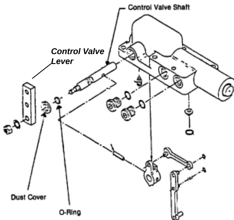
Eaton Manual Control Valve & Gasket
