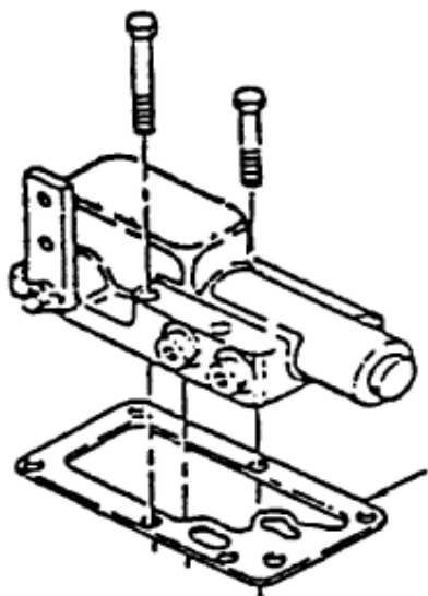
Eaton Manual Control Valve & Gasket
