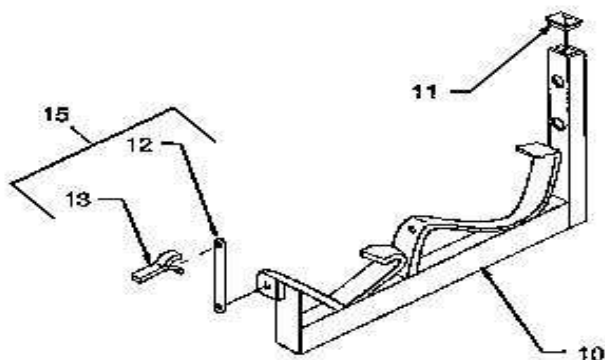
L STYLE BRACKET
