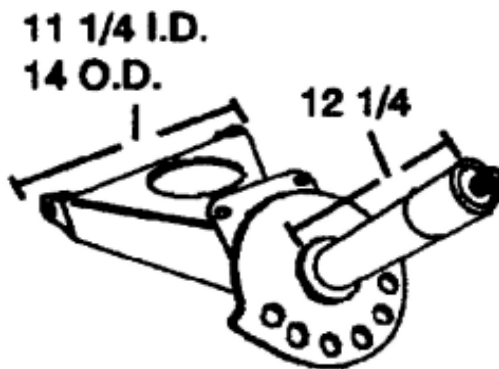
3/4" BUSHINGS
