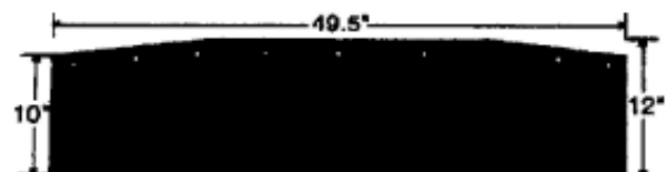
CB 1004 SMITH HOPPER BIB OEM # 29372
