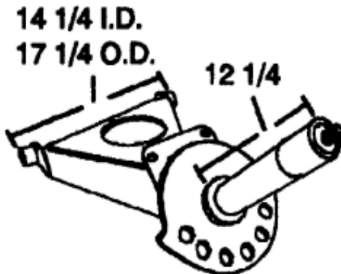
C 1023-A MTM # 560.150320 MTM Bushing (C 1032 Garlock Bushing) Pivot Arm Fits C 4002 Main Chute
