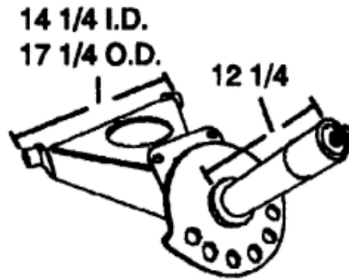
C 1023 MTM # 560.152305 MTM Bearing Pivot Arm Fits C 4002 Main Chute
