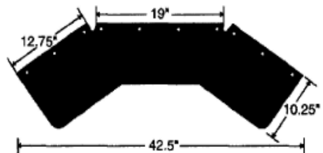
CB 1011 JAEGER HOPPER BIB OEM # 59533-1
