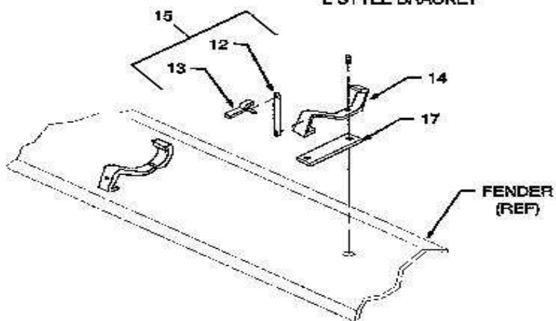
FENDER MOUNT BRACKET
